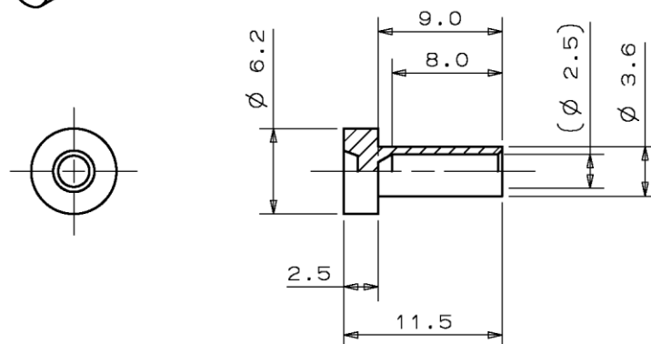
Figure 9 ⑧-1 Cap (Ferrule cap)
