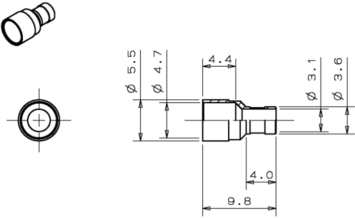
Figure 6 ⑤Crimping Ring
